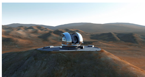
Figur 9. 3D computermodel af det planlagte 39m European Extremely Large Telescope (E-ELT; ESO).
